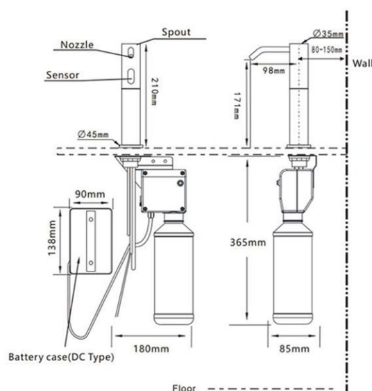
▲ DC (6V x Alkaline) Installation Instruction
