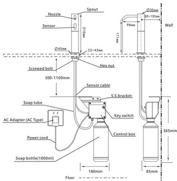
▲ AC (110-240V) Power Installation Instruction
